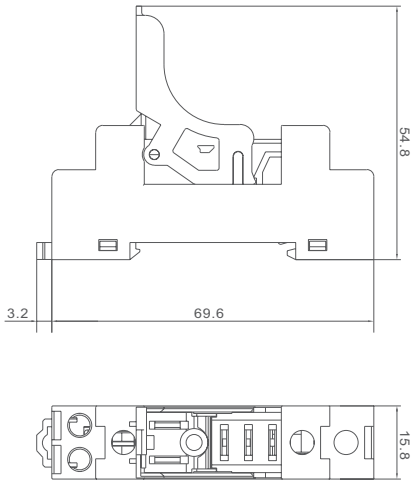
PCR-1C-T
