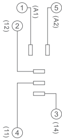
PCR-1C-T
