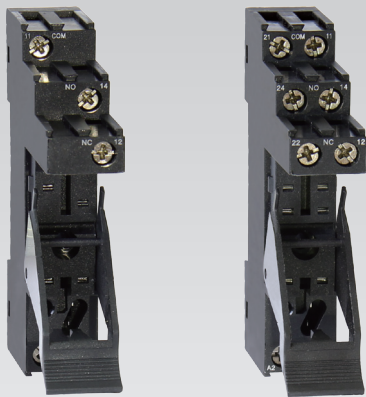
PCR-1C-S
