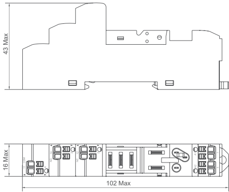
PCR-1C-K-DK
